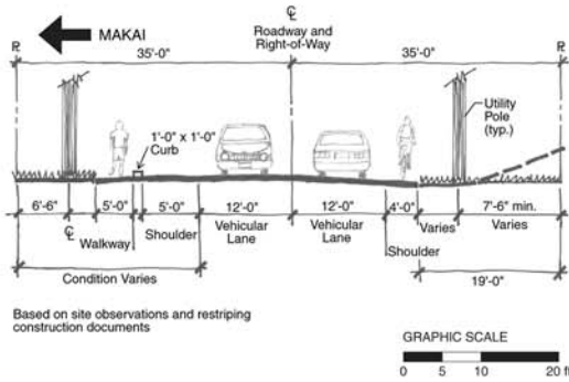
Kalaniana'ole Street Right-of-Way/Existing Conditions: Banyan Way to Kūhiō Street
