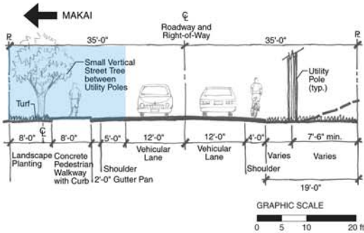
Kalaniana'ole Street Right-of-Way: Proposed Trail Improvement on Makai Side
