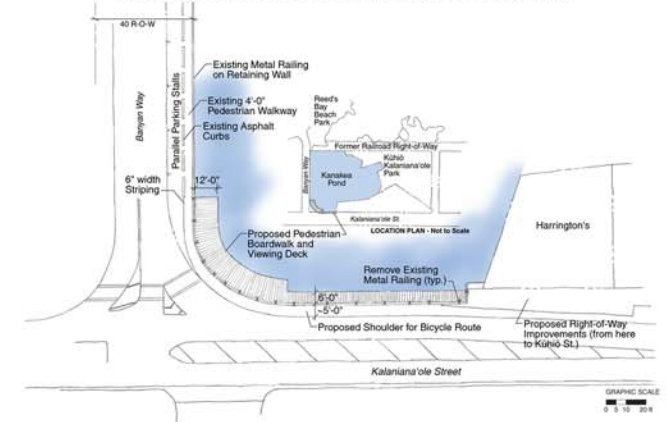
Kanakea Pond Proposed Boardwalk and Viewing Deck
