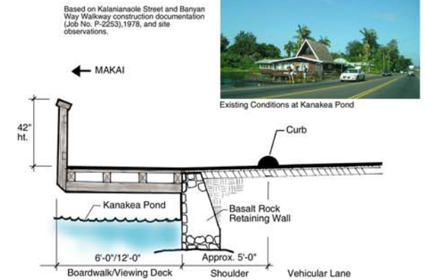
Kanakea Pond Proposed Pedestrian Board walk and Viewing Deck: Section
