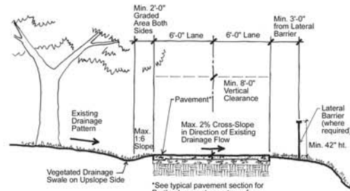
Two-Way Shared Use Path: Section
